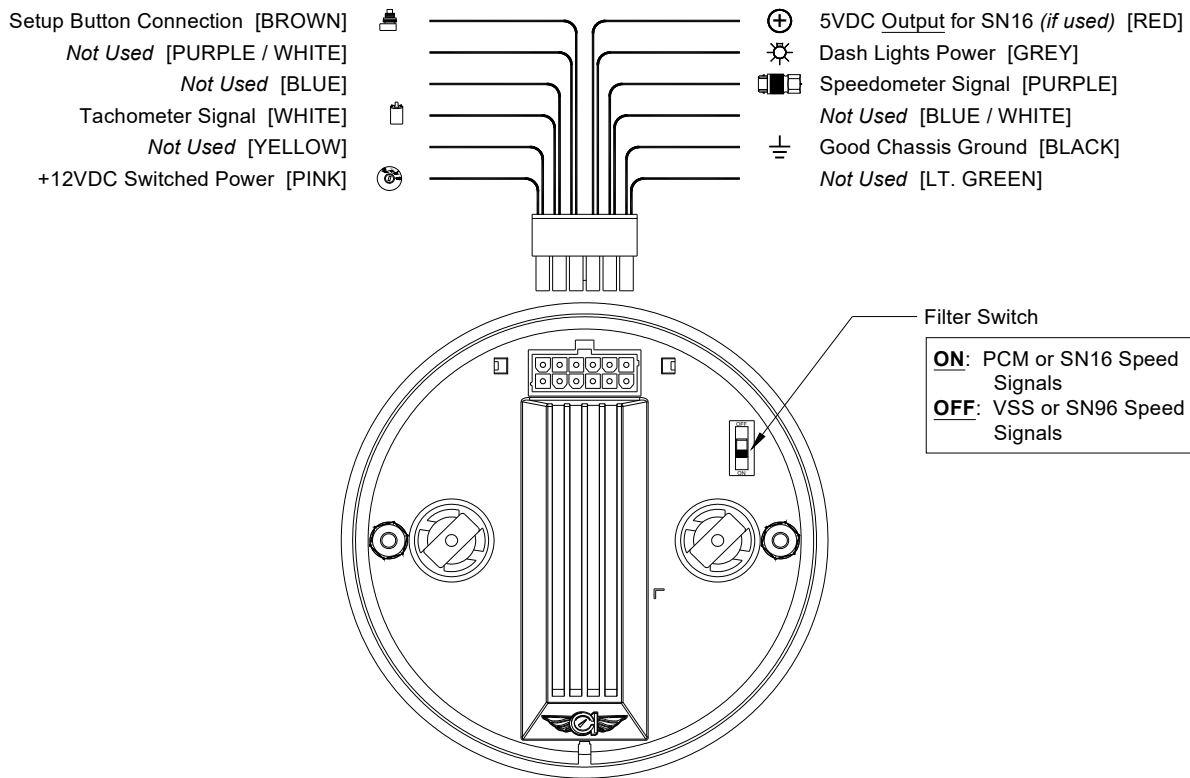
4 5/8" Speed-tachular Wiring
